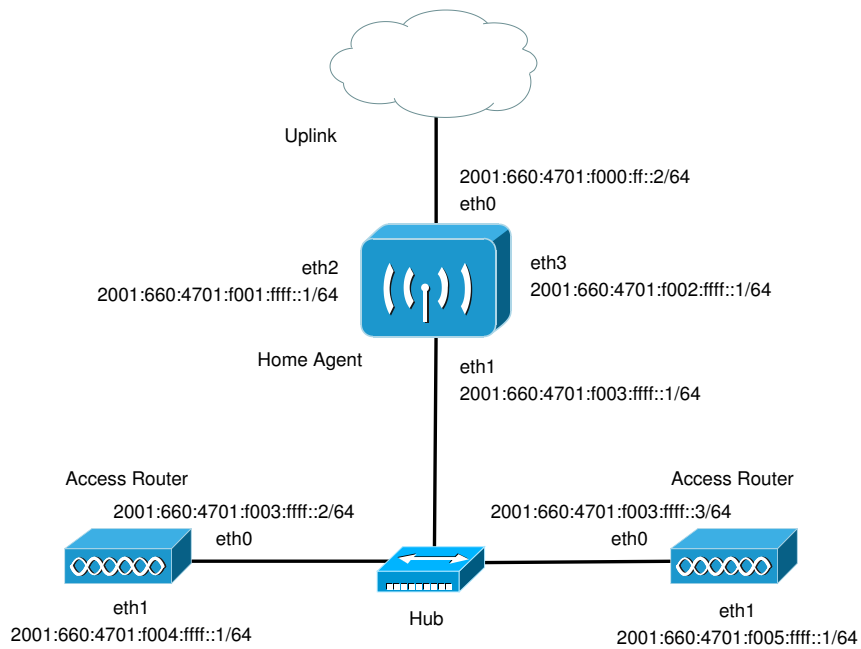
Figure 4.1: FMIPv6.org Testbed
